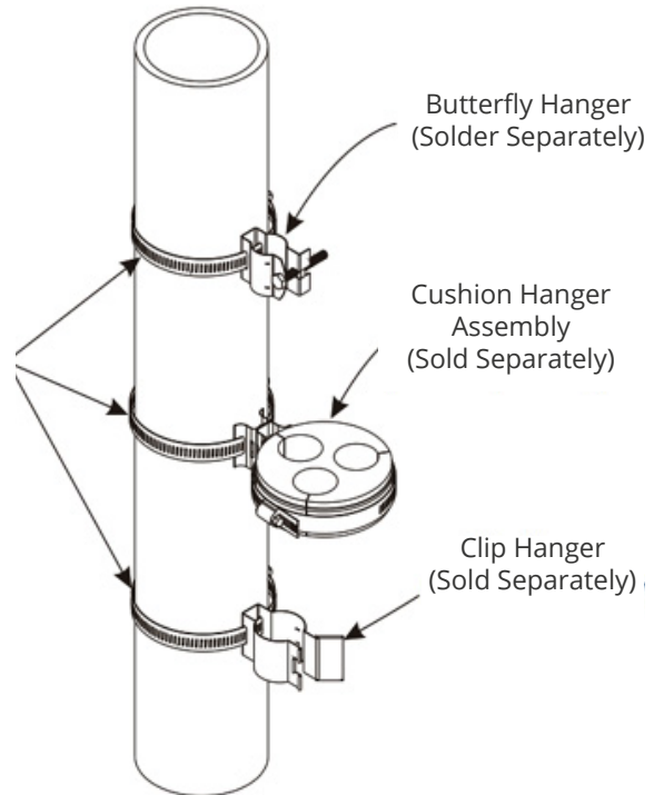
Round Member Adapter Kits (MAR-RMA200X Shown)
